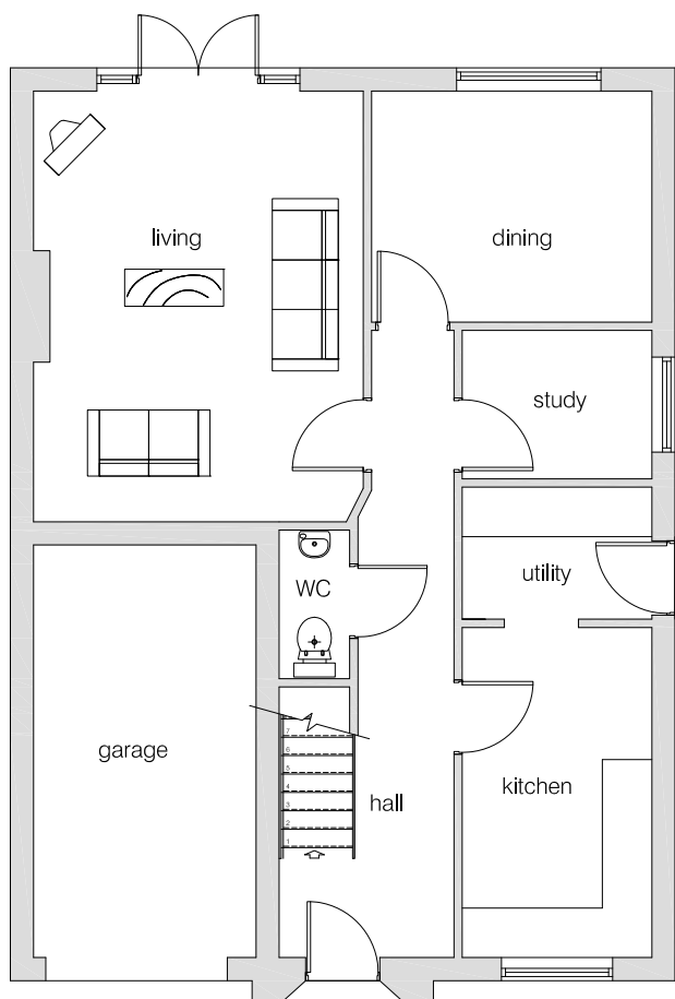
ground floor plan Total floor area = 1383 ft 2
