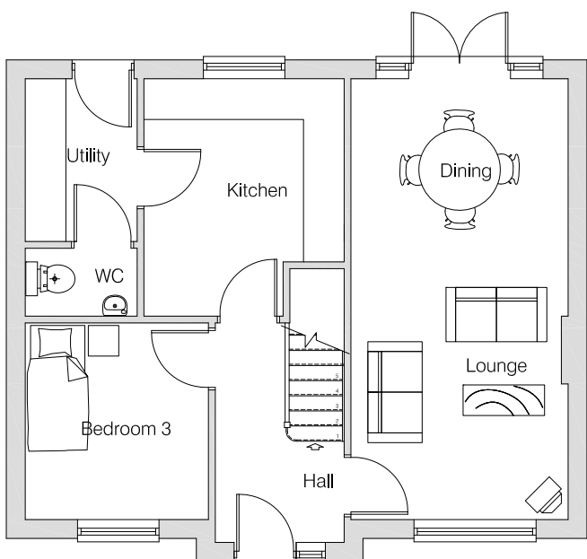
ground floor plan Total floor area = 973 sq.ft
